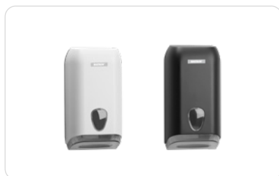
92582 Katrin Folded Toilet Tissue Dispenser - White 92605 Katrin Folded Toilet Tissue Dispenser - Black ABS-plast 1 stk. / kolli H: 307, B: 158, D: 133 (mm)
